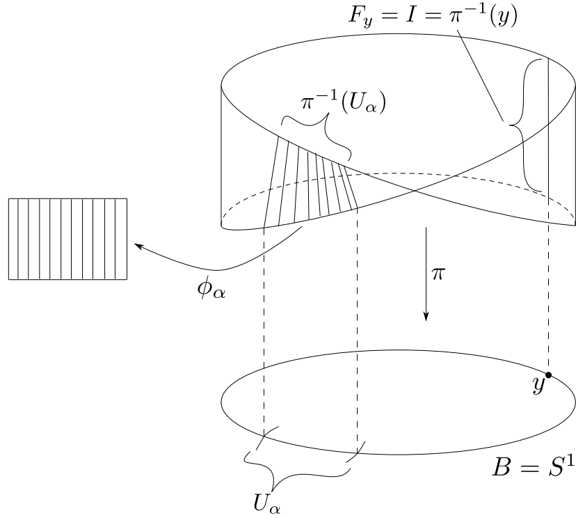
Figure 19: The Möbius strip is a fibre bundle with fibre I , base S^1 and structure group \mathbb{Z}_2 . The figure shows an open subset U_\alpha \in S^1 , \pi^{-1}(U_\alpha) and the local trivialisation \phi_\alpha : \pi^{-1}(U_\alpha) \rightarrow U_\alpha \times I . The fibre above a point y \in S^1 is F = I = \pi^{-1}(y) .
