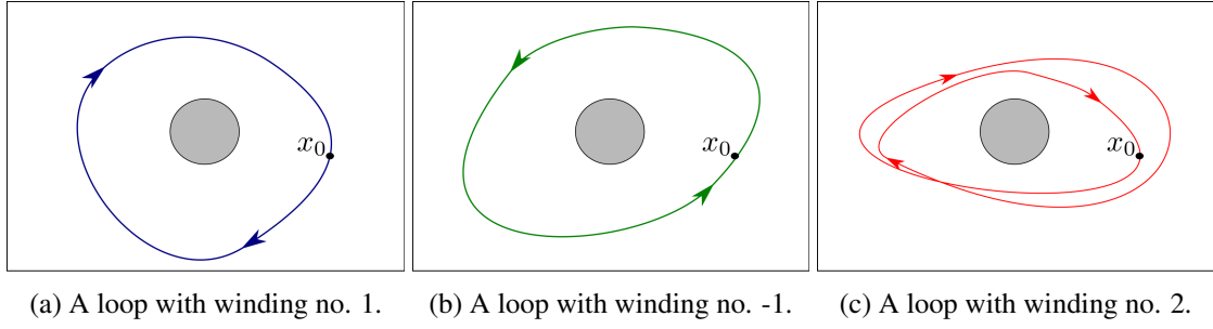
Figure 6: The punctured plane has a non-trivial first homotopy group \pi_1 \simeq \mathbb{Z} and hence homotopy classes of loops can be labelled by a winding number, counting how many times they wind the hole clockwise. The figures show three loops at x_0 belonging to different homotopy classes.
