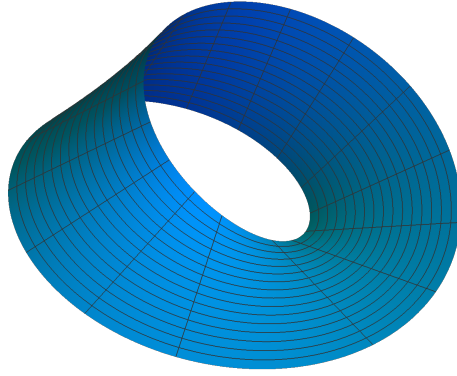
Figure 17: The Möbius strip is one of the simplest examples of a non-trivial fibre bundle.
