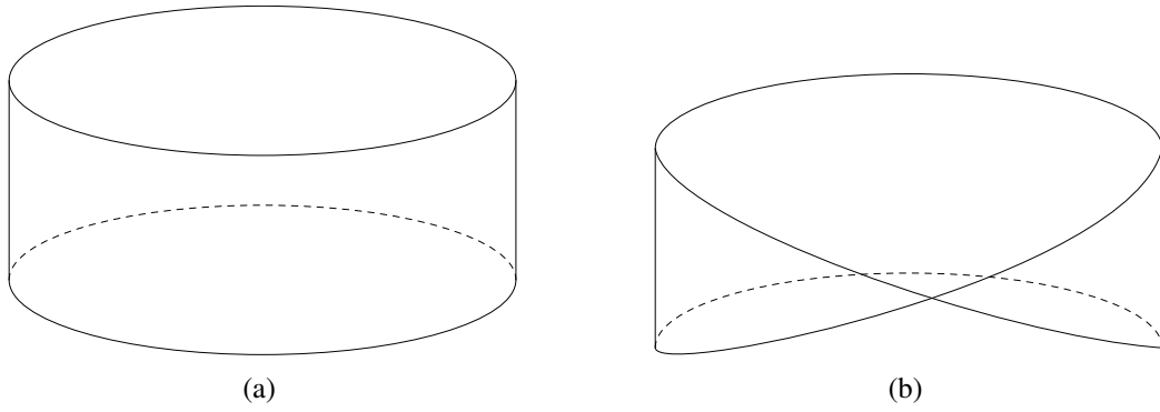
Figure 18: The cylinder shown in (a) is globally a product while the Möbius strip shown in (b) is not.
