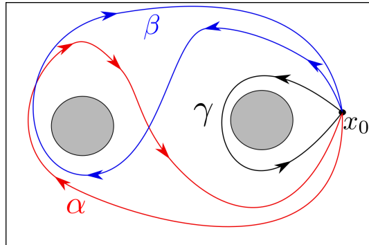
Figure 7: The plane with two punctures has a non-Abelian first homotopy group. This can be seen by considering the loops \alpha and \beta at x_0 which wrap the left hole while below / above the right hole and the loop \gamma at x_0 which wraps the right hole but not the left. Clearly, \alpha \neq \beta but \gamma^{-1} \star \alpha \star \gamma \simeq \beta from which it follows that the first homotopy group is non-Abelian.
