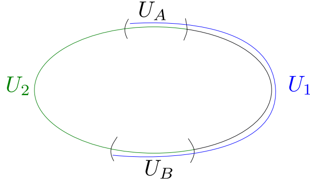
Figure 20: An open covering \{U_1, U_2\} of S^1 with intersections U_1 \cap U_2 = U_A \cup U_B .
